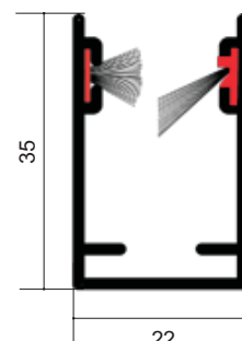
Security brush
