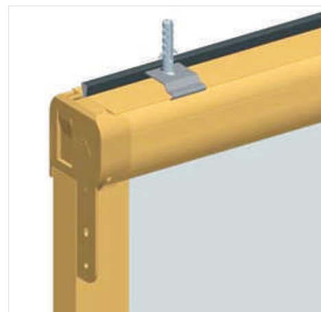
Upper fixing
